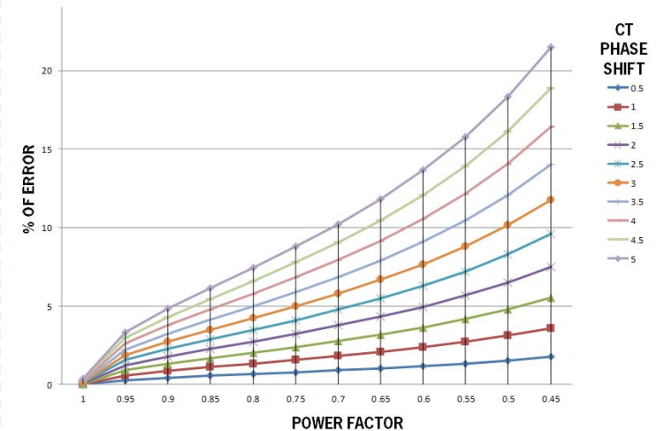
EFFECT OF CT PHASE ANGLE ERROR ON POWER MEASUREMENTS
